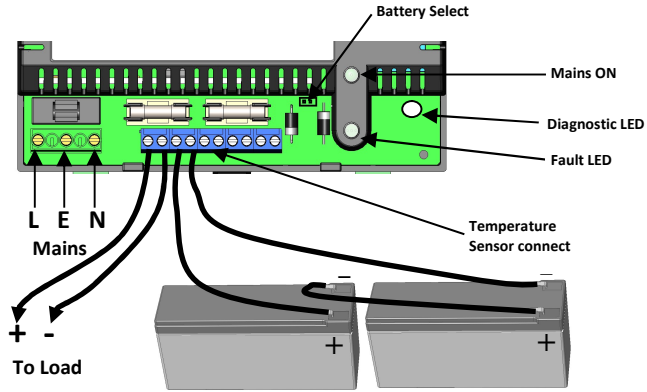
Figure 2 - Connections
