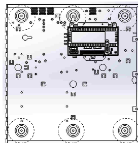
E enclosure
