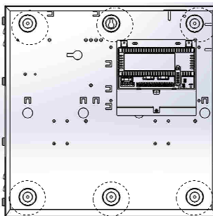
H enclosure
