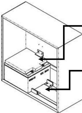
2402ST in H box with 24Ah batteries (battery omitted for clarity)
