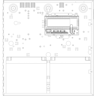
2402ST in H box with 38Ah batteries
