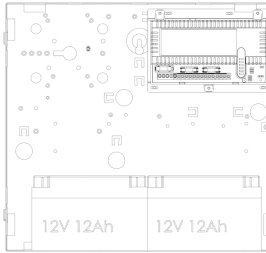
2402ST in K box with 12Ah batteries
